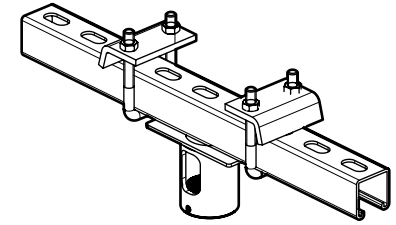
ISOMETRIC VIEW REFERENCE ONLY - NOT TO SCALE
