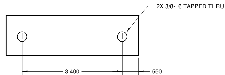
CHANNEL NUT - TOP VIEW
