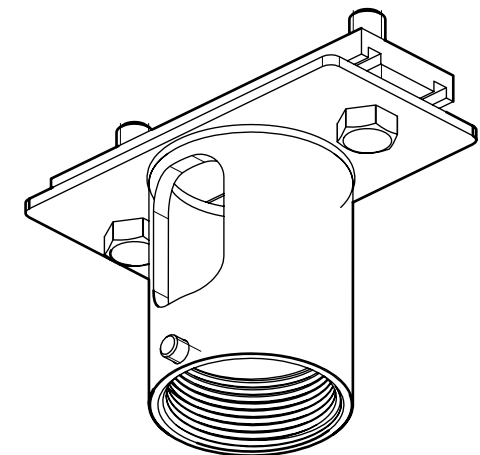
ISOMETRIC VIEW REFERENCE ONLY - NOT TO SCALE
