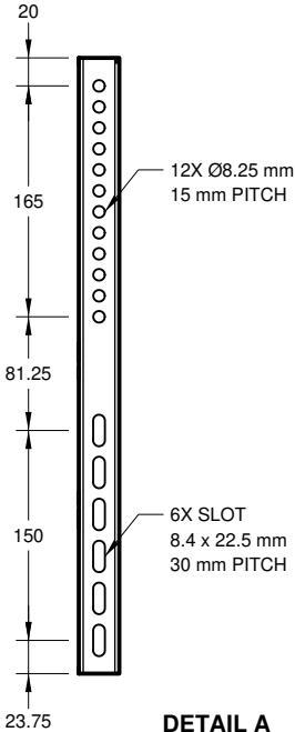
DETAIL A TV RAIL (BOTH) SIZES IN mm
