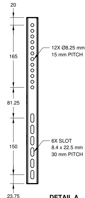
DETAIL A
