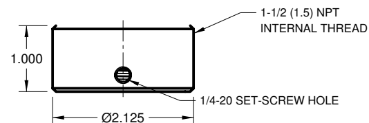
DETAIL B
