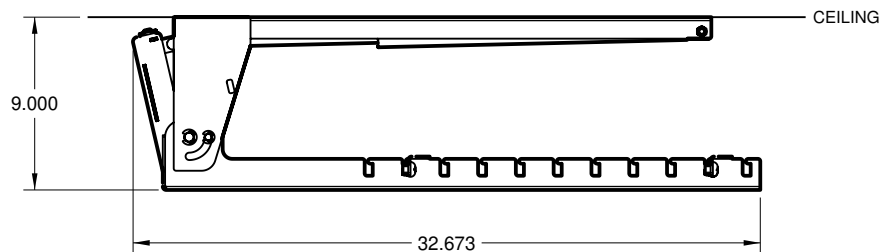
SIDE VIEW - FOLDED
