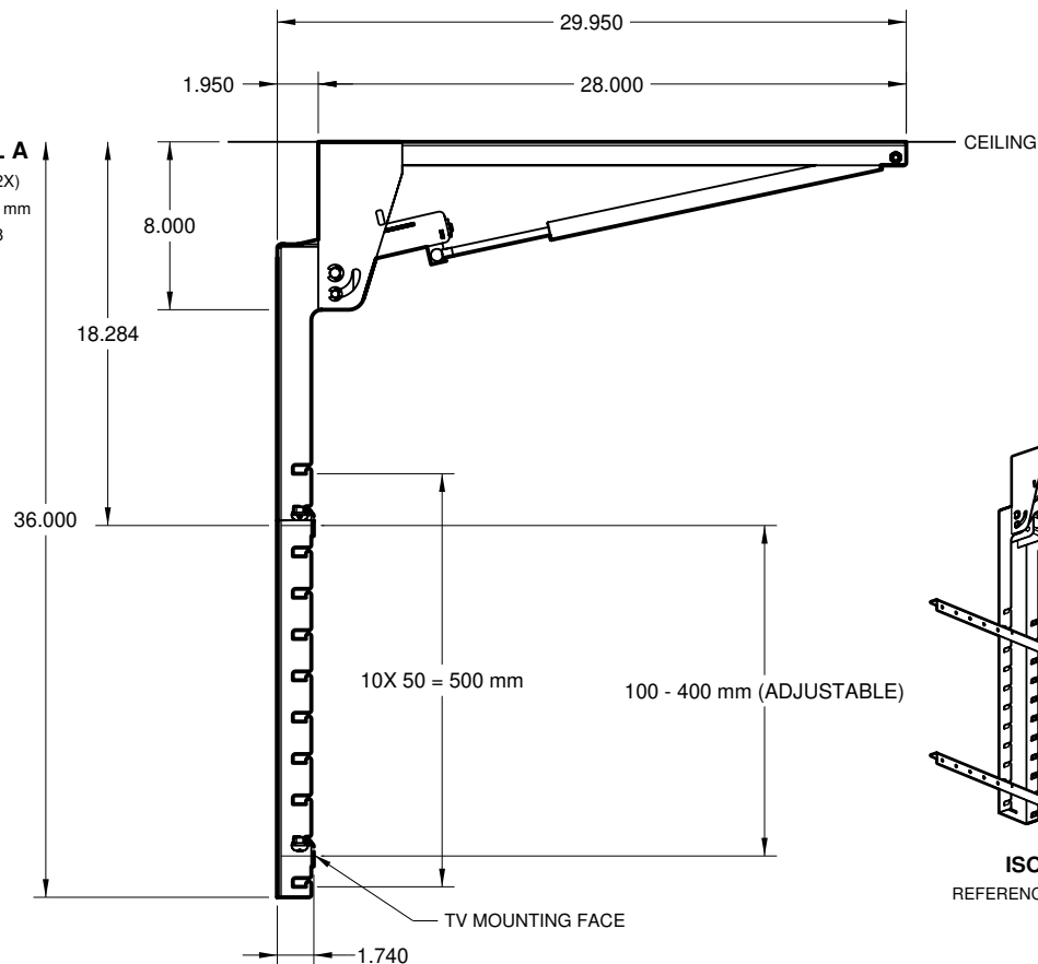
SIDE VIEW - UNFOLDED
