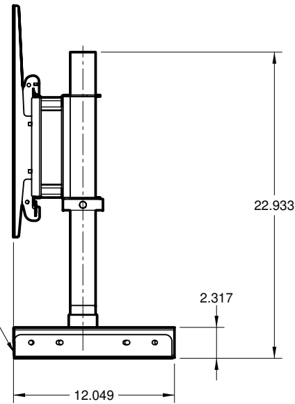
RIGHT SIDE VIEW - COLLAPSED
